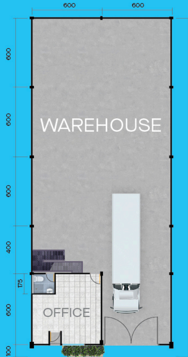
DENAH LANTAI 1
