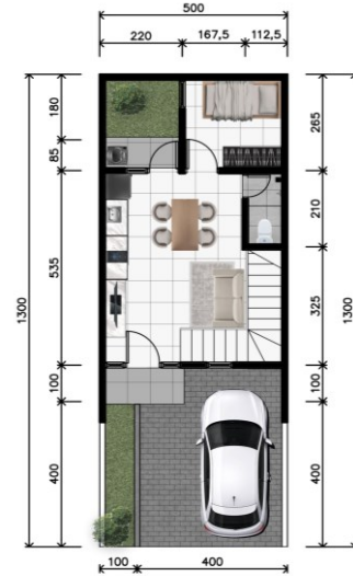
DENAH LANTAI 1 SKALA 1:100
