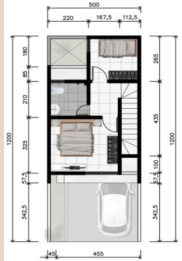
DENAH LANTAI 2 SKALA 1:100
