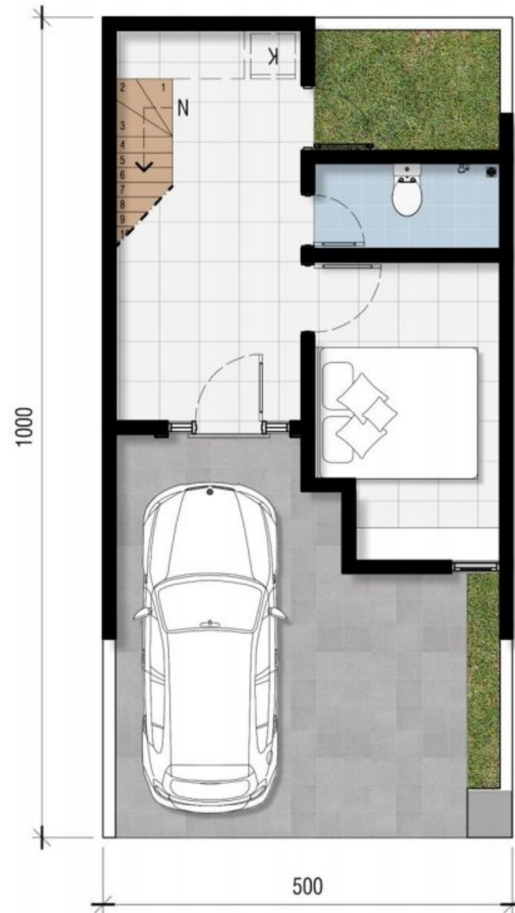
DENAH LT. 1
