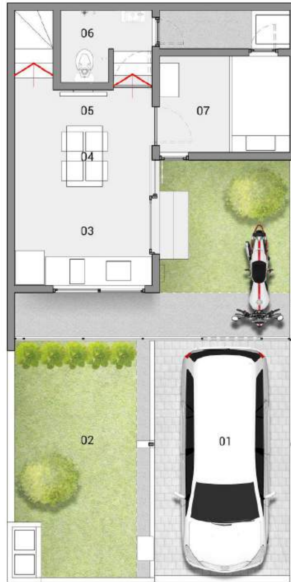
DENAH LANTAI 1
