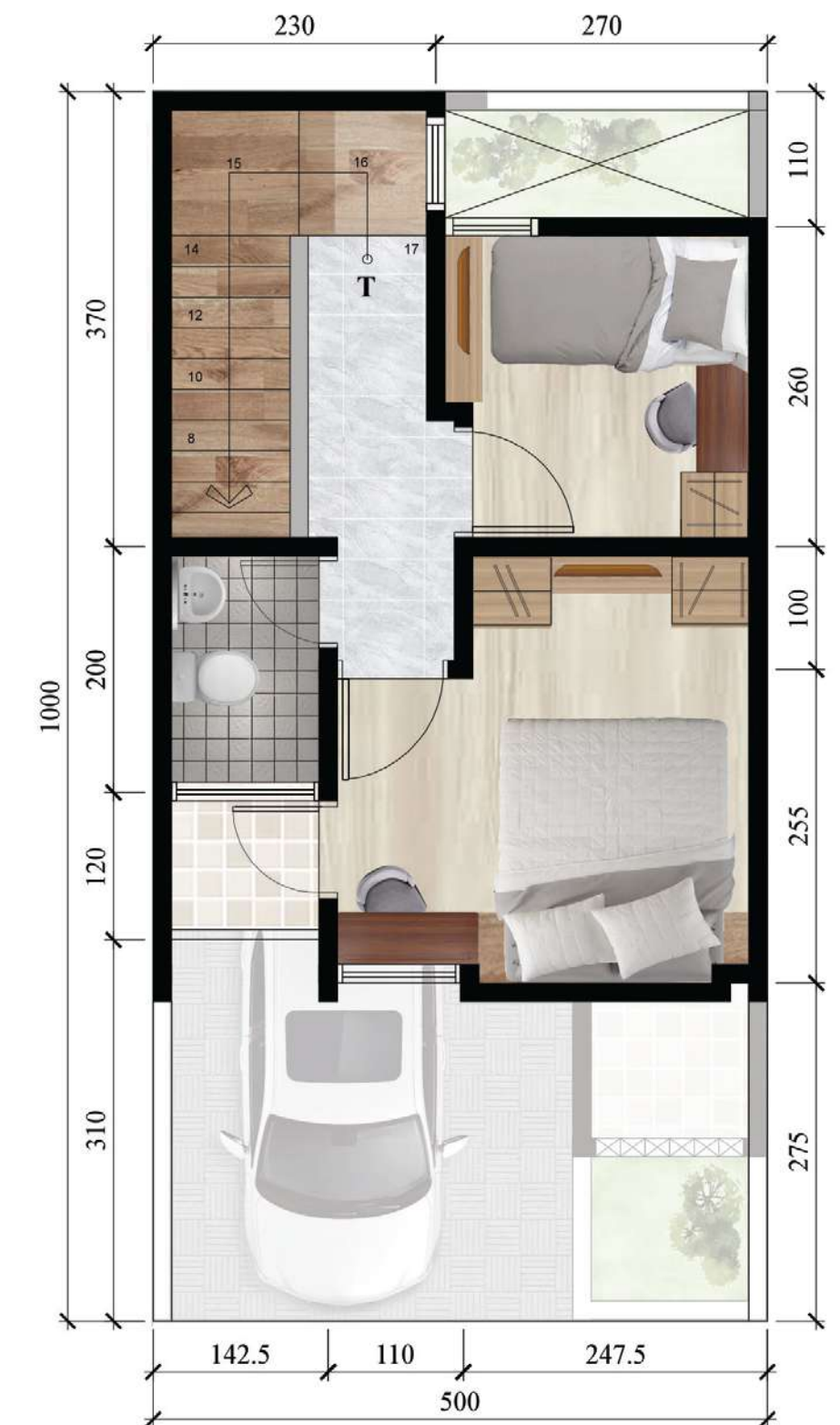
DENAH LANTAI 2
