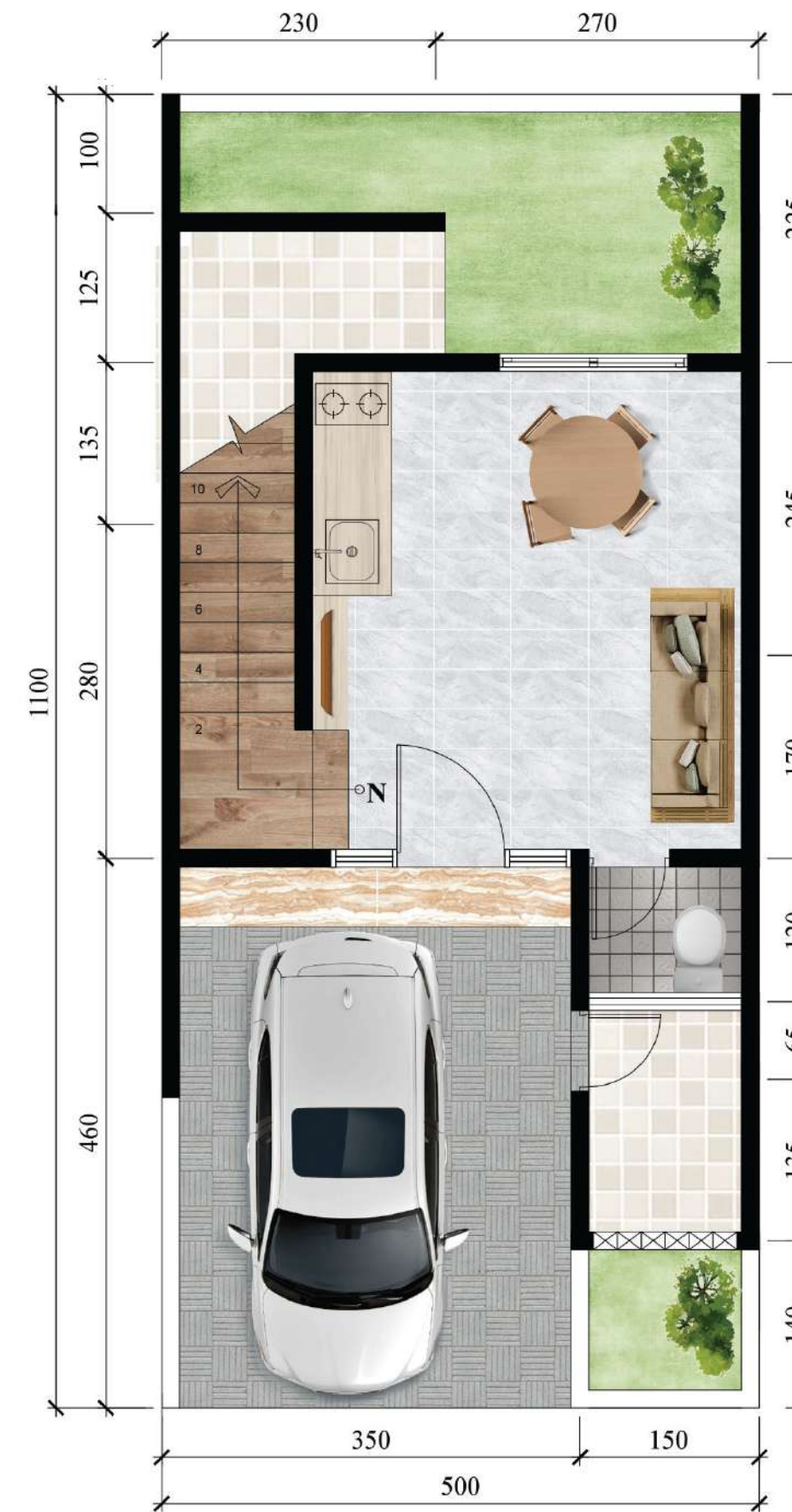
DENAH LANTAI 1
