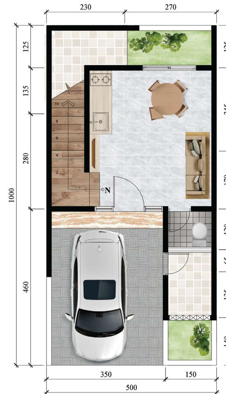
DENAH LANTAI 1
